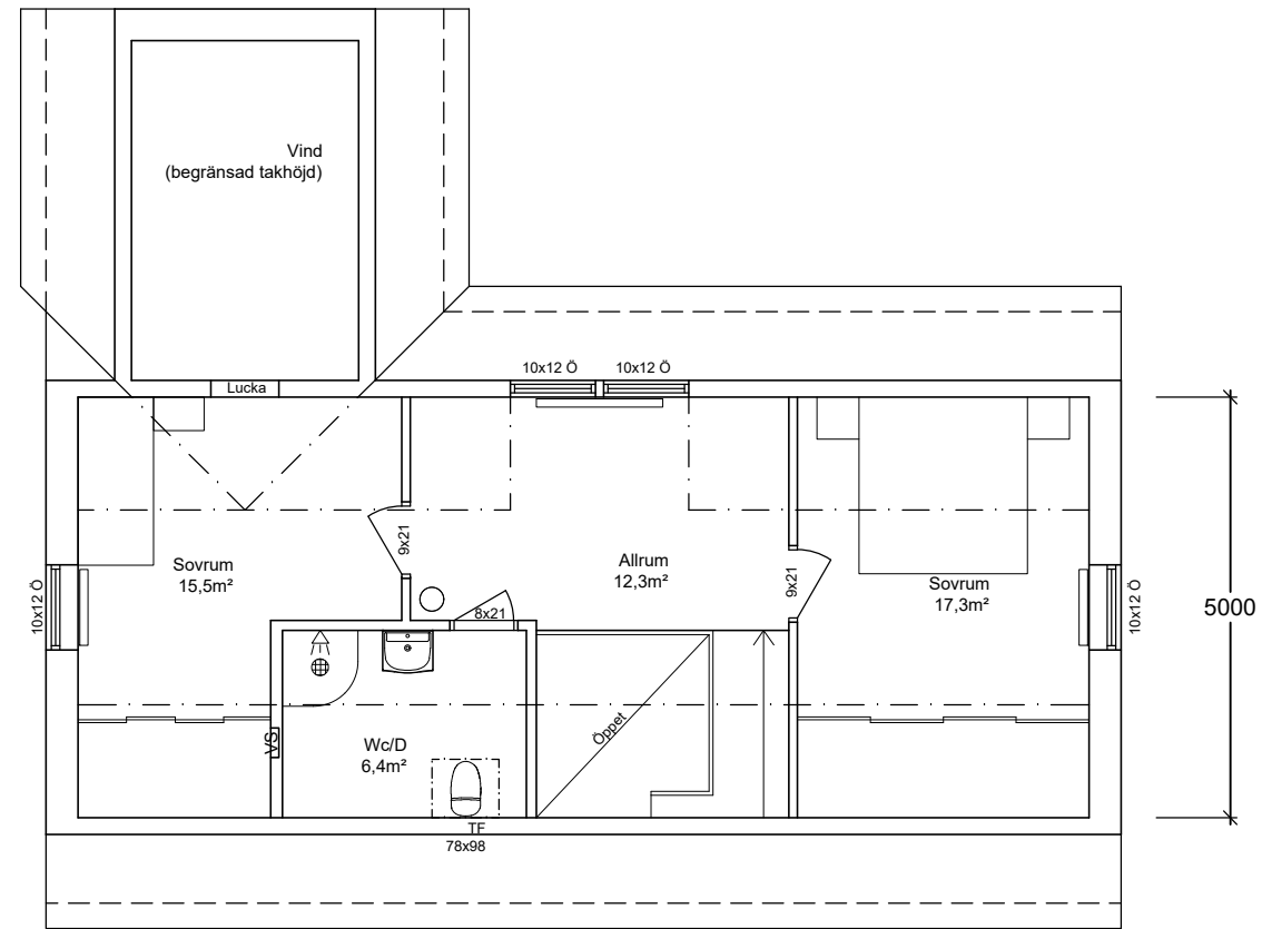
PLAN 2
